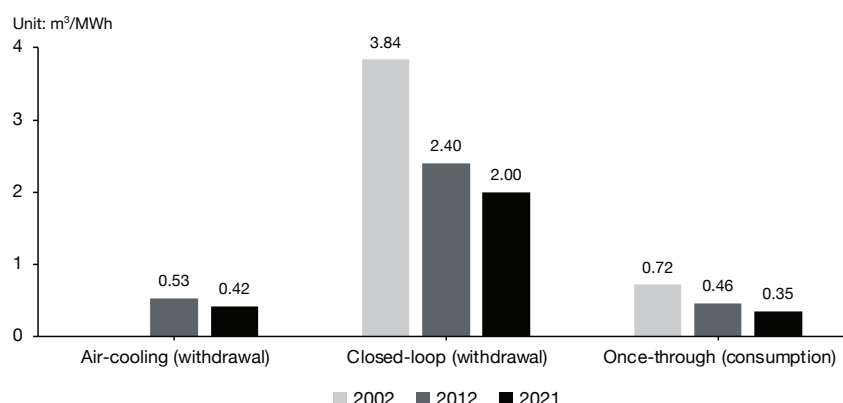
Norm of water use for thermal power
