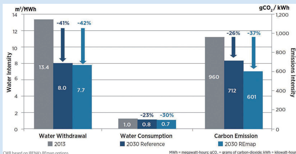
Water and carbon intensity of power generation (2013-2030)
