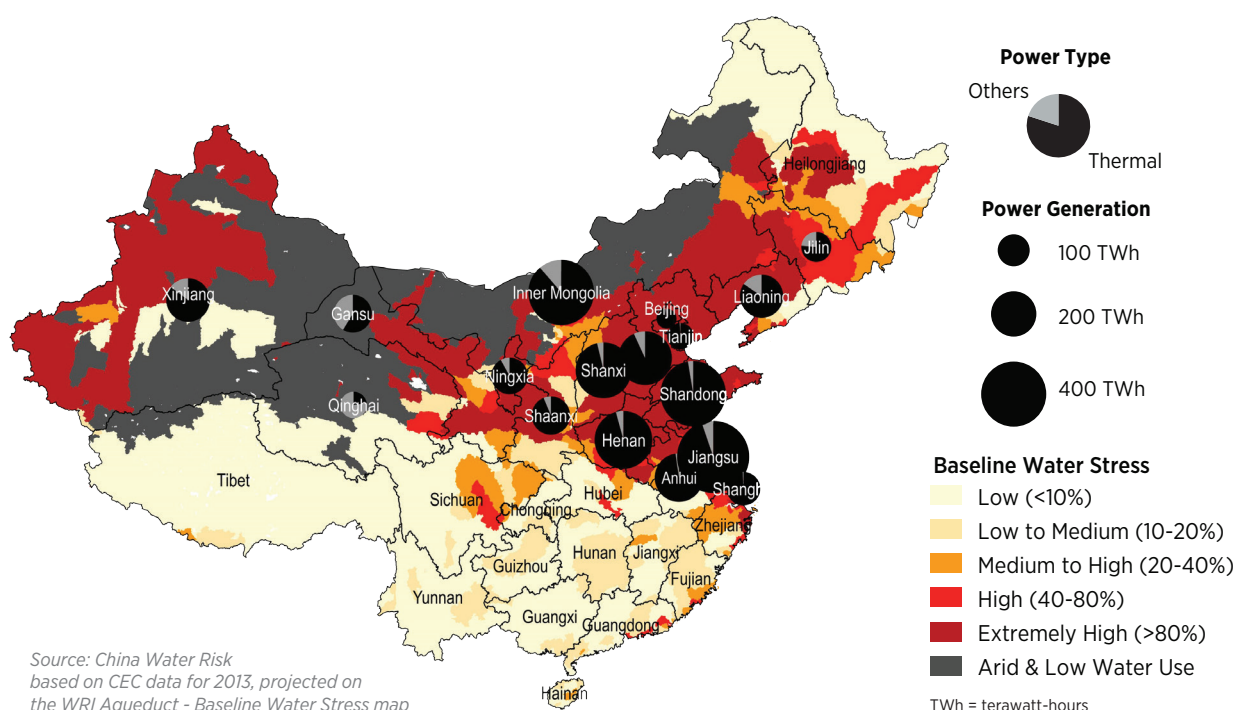
FIGURE 1: WATER-STRESSED AREAS AND THERMAL POWER GENERATION
