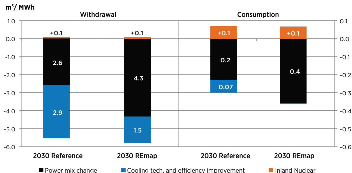
FIGURE 5: FACTORS IMPACTING WATER INTENSITY OF POWER (2013-2030)
